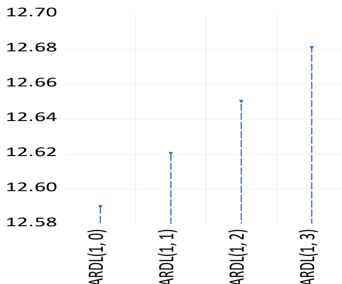
Akaike Information Criteria
