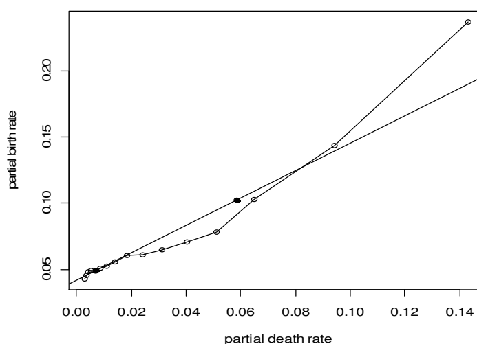
Figure 4 Plot of partial birth rates against partial death rates, females
