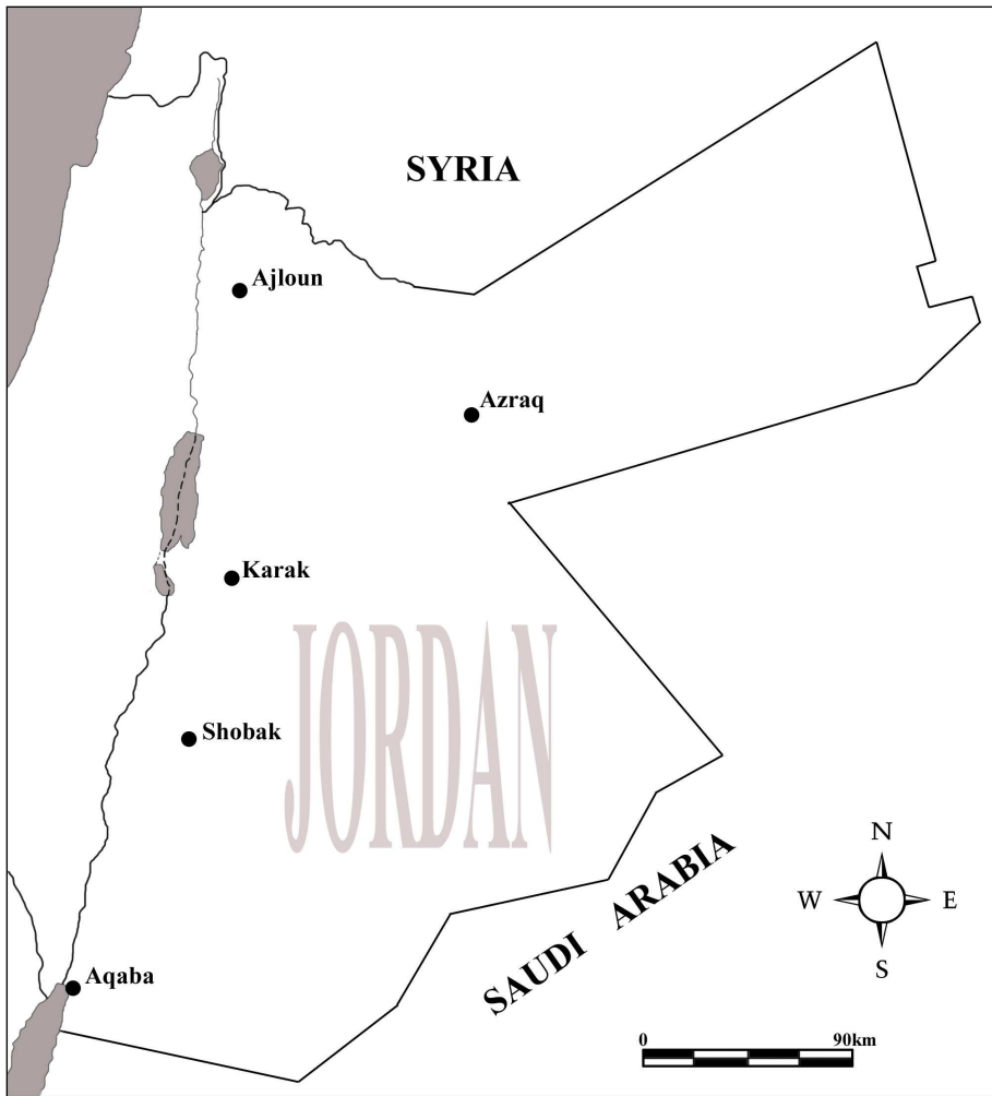
* Map of the Medieval Castles of Jordan (By the researcher).
